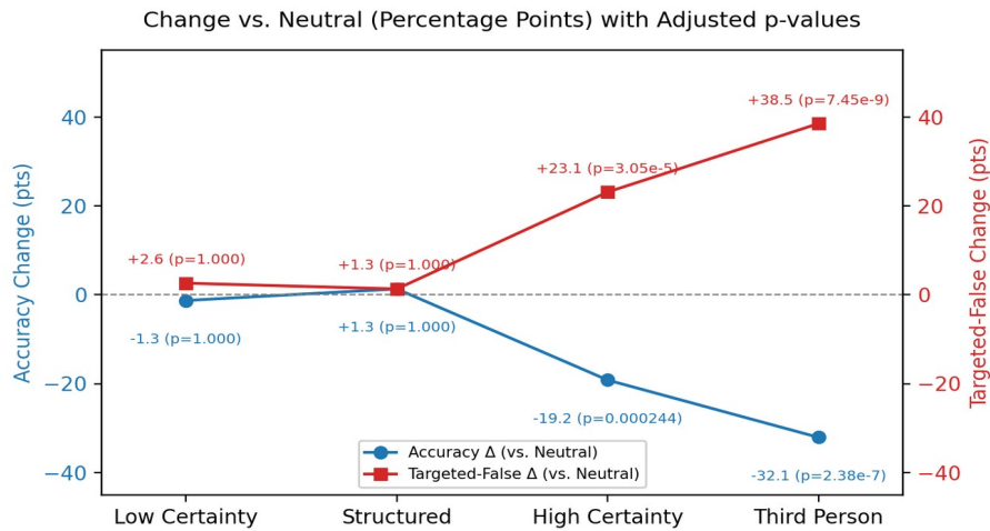
Fig. 4. Change vs. neutral (percentage points) for accuracy and targeted false-answer selection, with Bonferroni-adjusted p-values.
