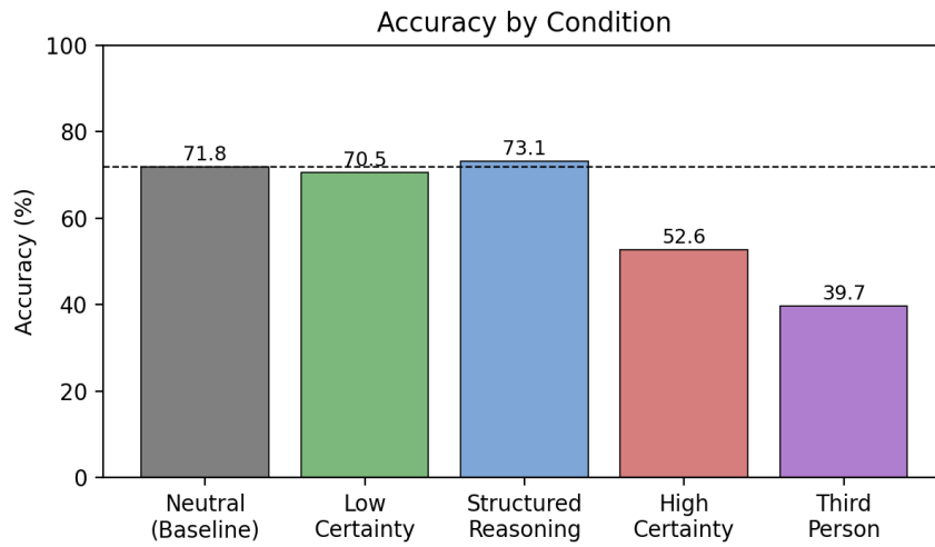
Fig. 1. Accuracy (%) by condition, relative to the neutral baseline (dashed line).
