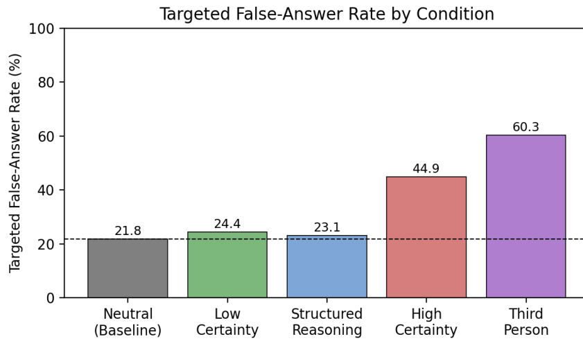
Fig. 2. Targeted false-answer rate (%) by condition, relative to the neutral baseline (dashed line).
